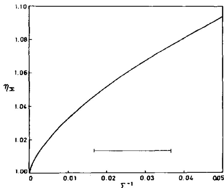
Fig. 1. Configuration interaction ratio ( \eta_{\Sigma} ) dependence on reciprocal ligand field strength ( \Sigma^{-1} ). The experimentally observed range of ligand field strengths in spin-paired d^6 octahedral complexes (—).
