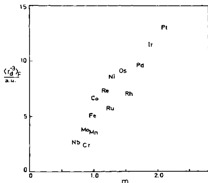
Fig. 11. Free-ion (atom) d -electron inverse cube distance ( \langle r_d^{-3} \rangle_F , Table 12) correlation with metal complex excitation energy parameter m [142] for d^6 transition metals.
