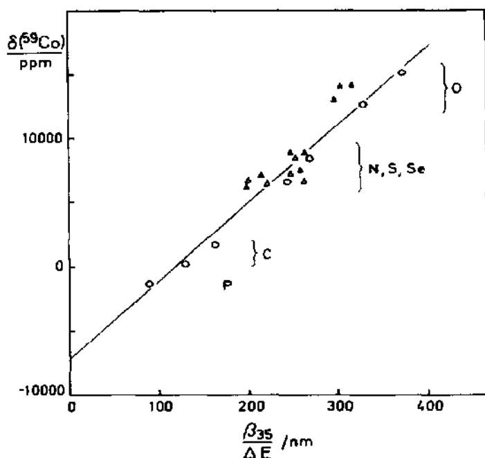
Fig. 6. Correlation of ^{59}\text{Co} NMR chemical shifts with ^1A_{1g} \rightarrow ^1T_{1g} electronic transition wavelength ( 1/\Delta E ) multiplied by nephelauxetic ratio \beta_{35} for ortho-axial (○) and non-ortho-axial (△) cobalt(III) complexes.
